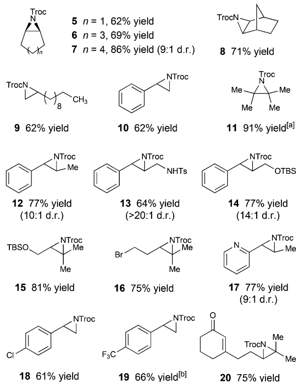
Figure 1. Scope of aziridination products available by photocatalytic activation. Reactions were conducted using alkene (0.40 mmol) in degassed solvent and irradiated with a 15 W blue LED flood lamp for 20 h. Yields represent the averaged values from two reproduced experiments. [a] Isolated as a 13:1 mixture of aziridine to imine (see the Supporting Information for more information). [b] Reaction irradiated for 30 h. Troc = 2,2,2-trichloroethoxycarbonyl; Ts = tosylate; TBS = tert -butyldimethylsilyl.
